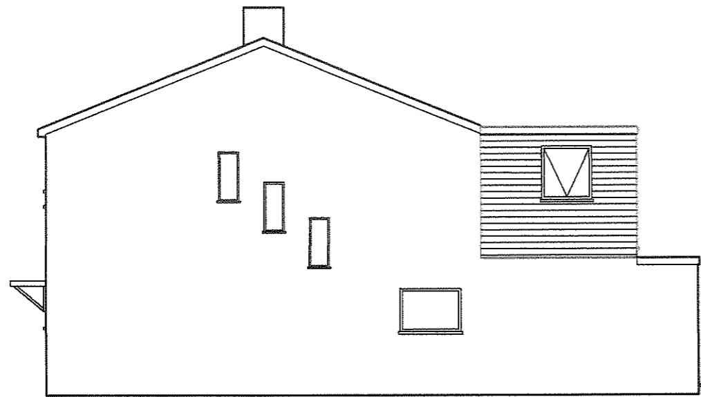
Side Elevation (East)
